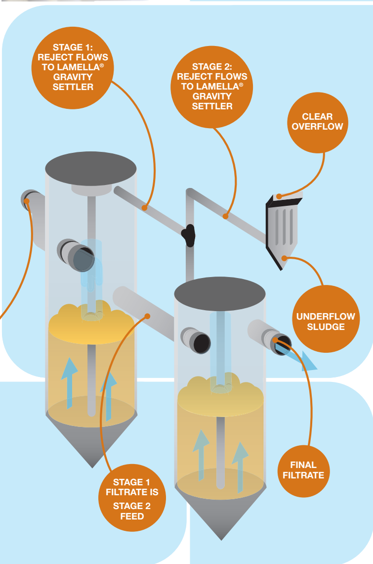
Inside a DynaSand D2® filter
