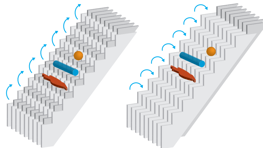
2. Movable lifting blades rotate upwards to lift the mat step-by-step.
